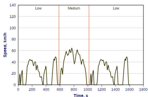
WLTC cycle for Class 1 vehicles
