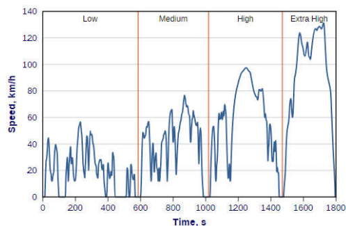
WLTC cycle for Class 3b vehicles
